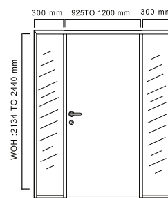
Single leaf with double side glass
