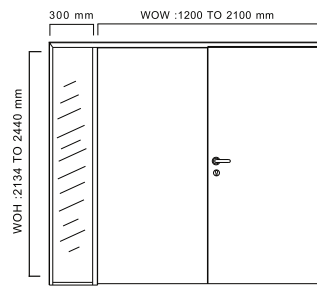
Double Leaf with Single side glass
