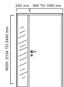
Single leaf with single side glass
